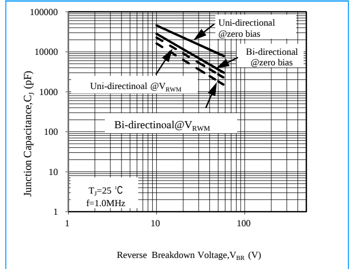
Figure 6-Typical Junction Capacitance
