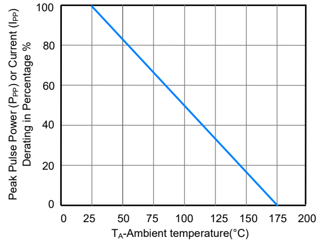
Figure 2-Pulse Derating Curve
