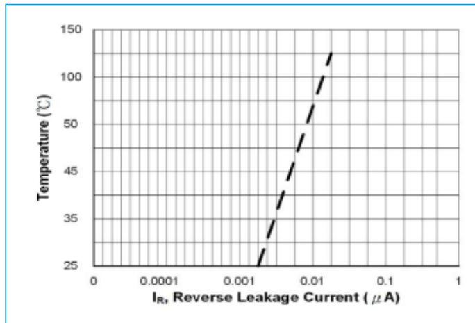
Fig5. Typic Reverse Leakage vs. Temperature
